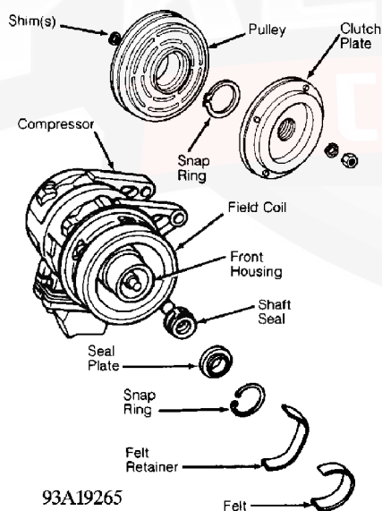
Fig. 13: Exploded View Of Compressor (Nippondenso 10-Cylinder)
