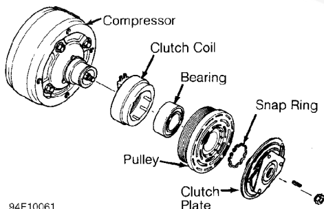
94F10061 Fig. 8: Exploded View of Compressor (Harrison R4 4-Cylinder)
