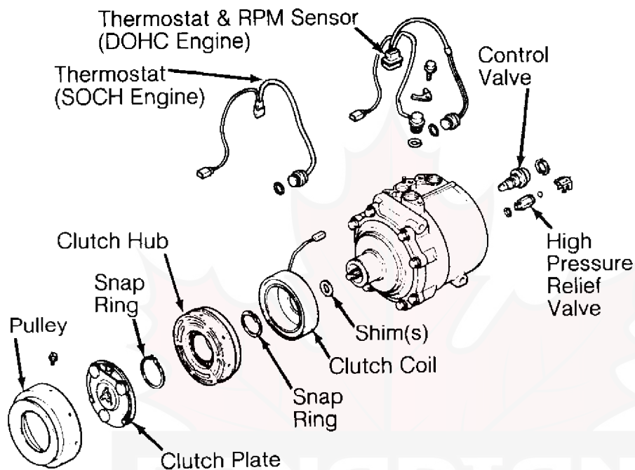
94A10066 Fig. 16: Exploded View Of Compressor (Sanden Scroll) Courtesy of Chrysler Corp.
